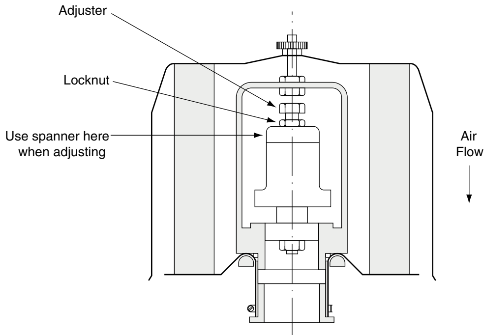
Diagram 2: Diagram showing D35BF-35 Valve.
